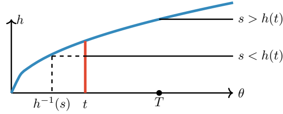
Figure 9: The top horizontal line is the belief’s support of an agent whose initial posterior mean is above T . The bottom horizontal line is the belief’s support of an agent whose initial posterior mean is below T , and hence at time t it is exactly T .
